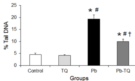
Fig. 5. Thymoquinone (TQ) protected against lead (Pb)-induced brain DNA damage (as % tail DNA) in rats for five-week treatment period. Each bar represents the mean \pm SEM of eight rats. *, P < 0.05 vs. control; #, P < 0.05 vs. TQ; †, P < 0.05 vs. Pb (One-way ANOVA and Tukey's post-hoc test)
