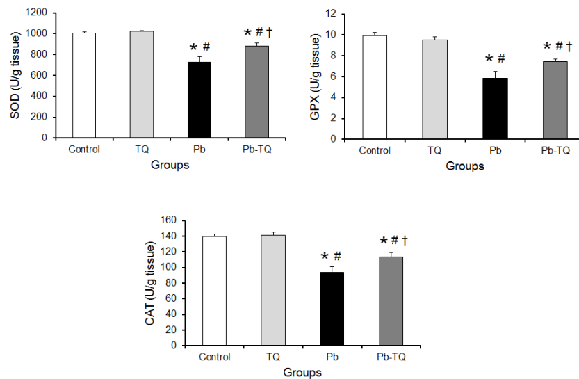
Fig. 2. Thymoquinone (TQ) protected against Pb-induced superoxide dismutase (SOD), glutathione peroxidase (GPX), and catalase (CAT) brain activities alteration in rats for five-week treatment period. Each bar represents the mean \pm SEM of eight rats. *, P < 0.05 vs. control; #, P < 0.05 vs. TQ; †, P < 0.05 vs. Pb. (One-way ANOVA and Tukey's post-hoc test)
