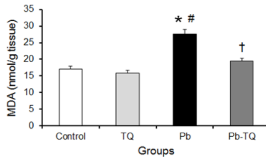
Fig. 4. Thymoquinone (TQ) protected against lead (Pb)-induced malondialdehyde (MDA) brain overproduction in rats for five-week treatment period. Each bar represents the mean \pm SEM of eight rats. *, P < 0.05 vs. control; #, P < 0.05 vs. TQ; †, P < 0.05 vs. Pb (One-way ANOVA and Tukey's post-hoc test)
