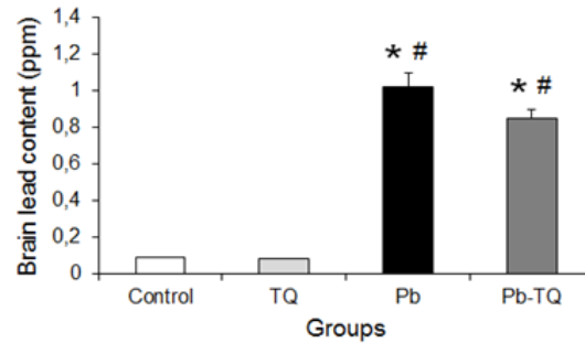
Fig. 1. Thymoquinone (TQ) had no effect on brain lead (Pb) level in rats for five-week treatment period. Each bar represents the mean \pm SEM of eight rats. *, P < 0.05 vs. control; #, P < 0.05 vs. TQ (One-way ANOVA and Tukey's post-hoc test)
