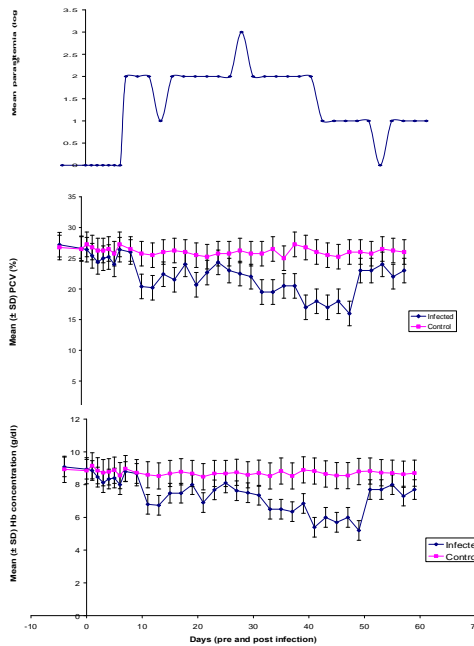
Figure 2: Mean PCV, Haemoglobin concentrations in relation to parasitaemia in Savannah brown Bucks
