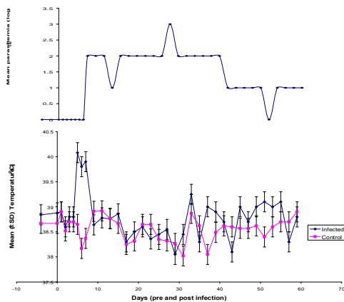
Figure 1: Mean parasitaemia in relation to rectal temperature in Savannah brown Bucks
