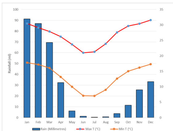
Figure 2 25-year climate data for Windhoek presented per month.
