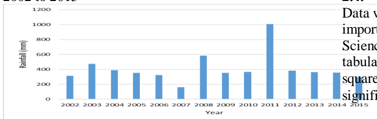
Figure 1 Total annual rainfall at Neudamm farm from 2002 to 2015
