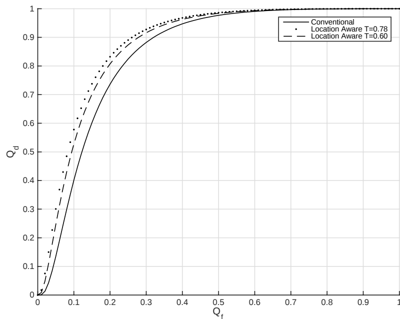
Figure 6. ROC comparison of proposed location-aware scheme and conventional hard combining scheme under Gaussian channel when the number of cooperative users = 30 for different trust values.
